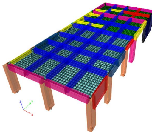
Temple Building
