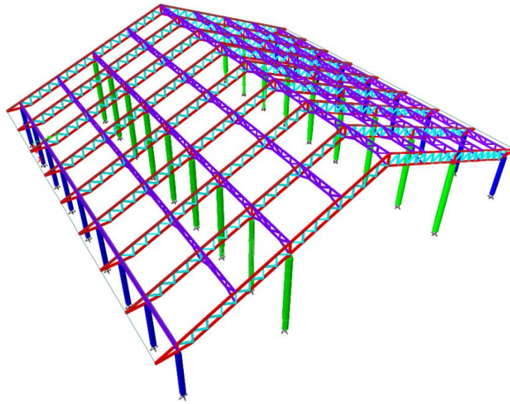
Temple Building
