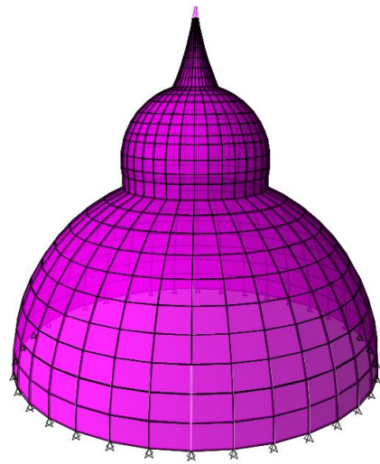
Temple Dome
