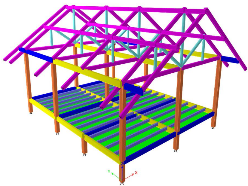
Timber House
