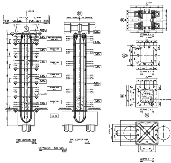
U tendon for Pier
