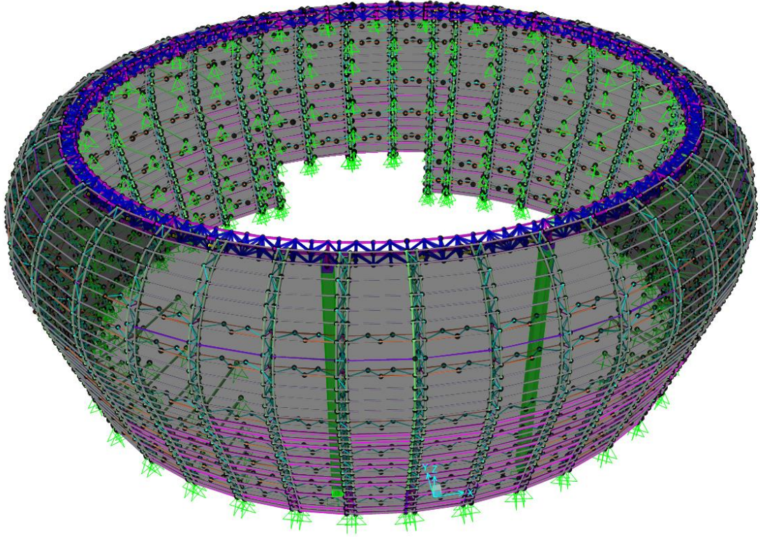
Façade Structure
