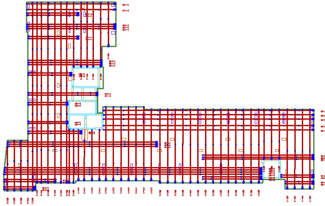
Post tension slab of building 19 story
