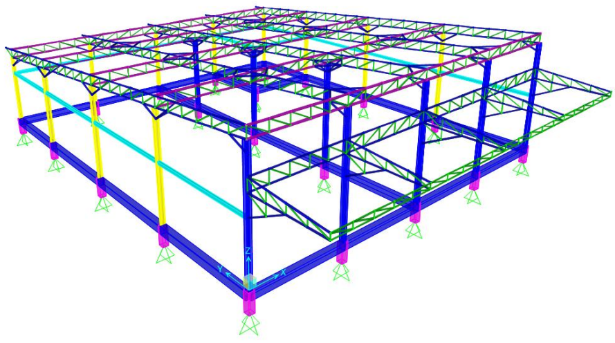
Warehouse
