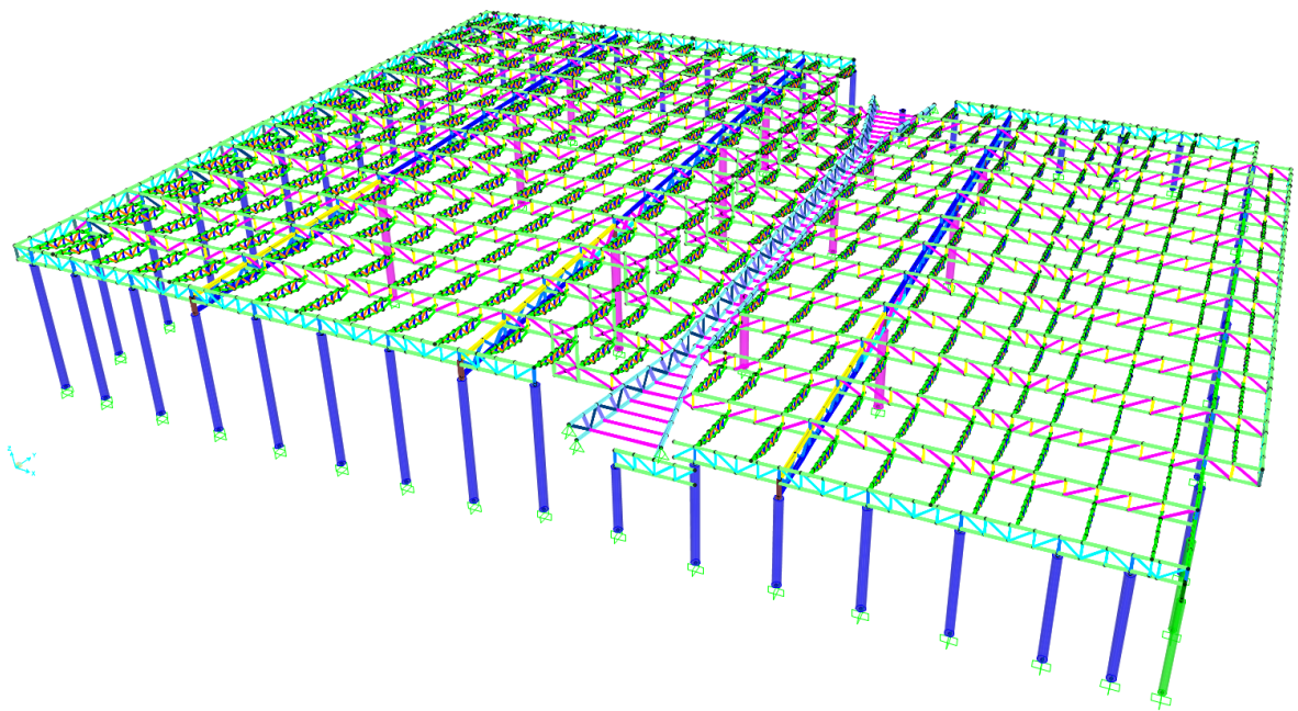
Terminal Building
