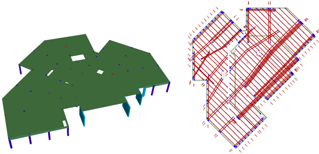
Post tension slab of building 8 story
