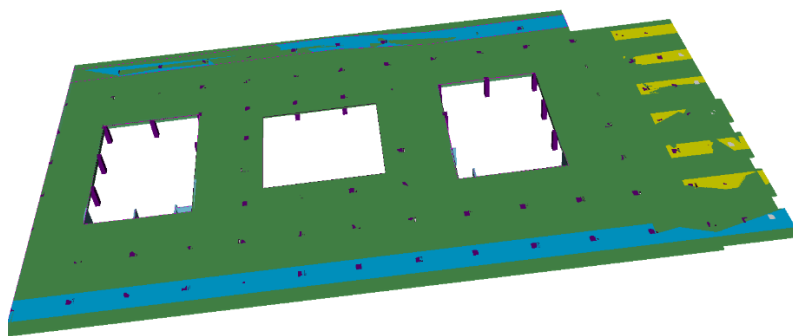
Post tension slab
