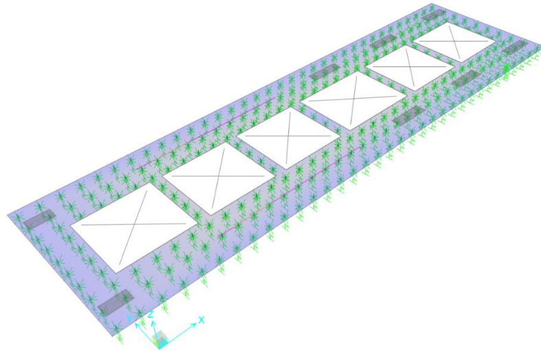
Foundation supports the machine
