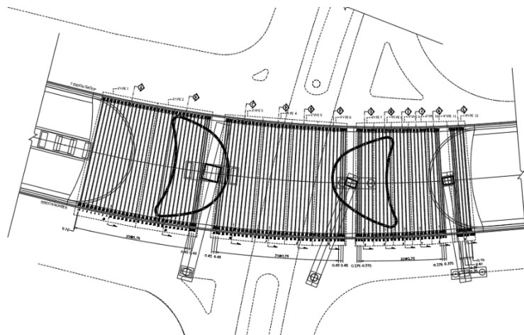
Master Plan for tunnel
