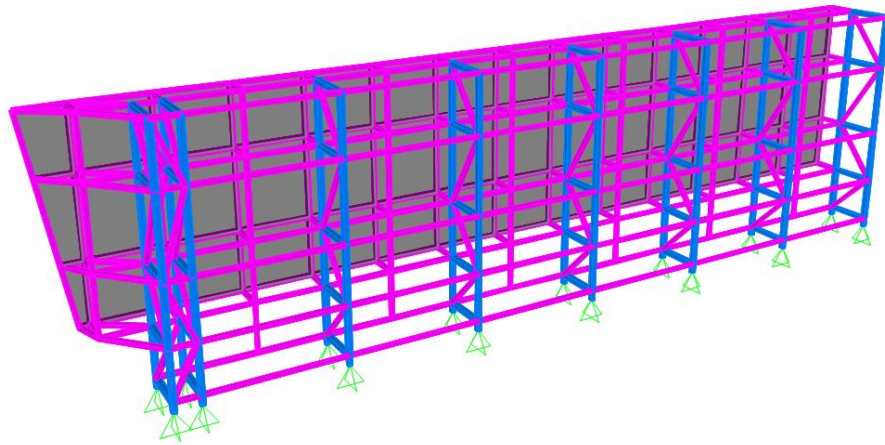
Cladding Structure
