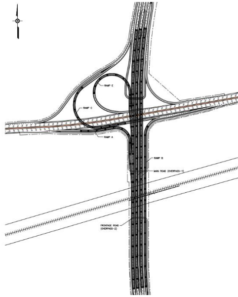
Master Plan for ring road
