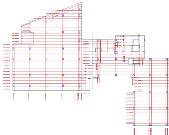
Post tension slab of building 11 story
