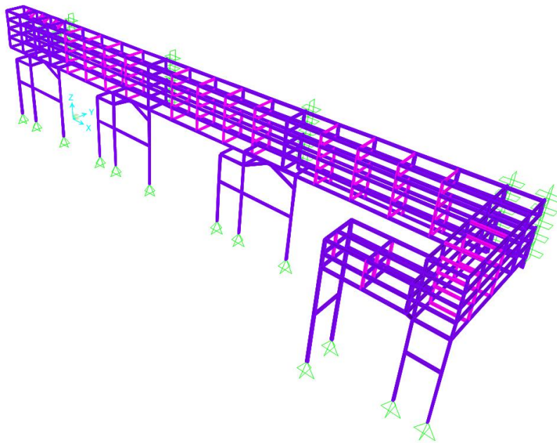
Steel Structure
