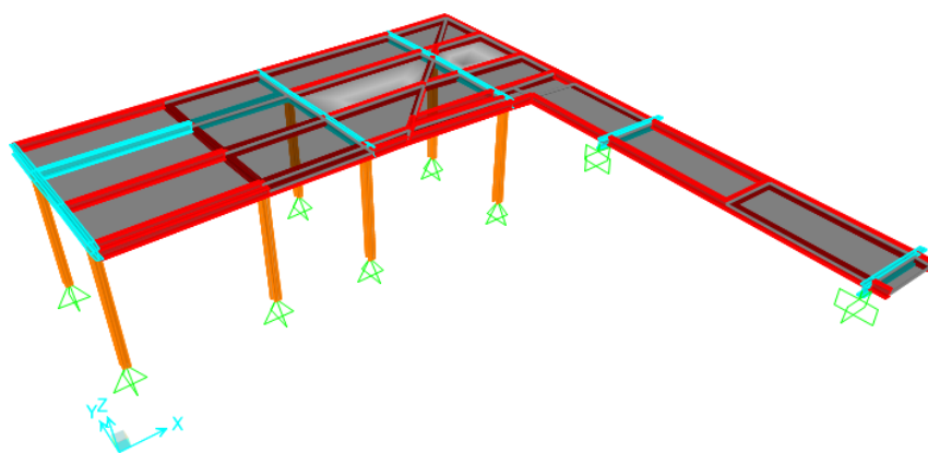
Canopy
