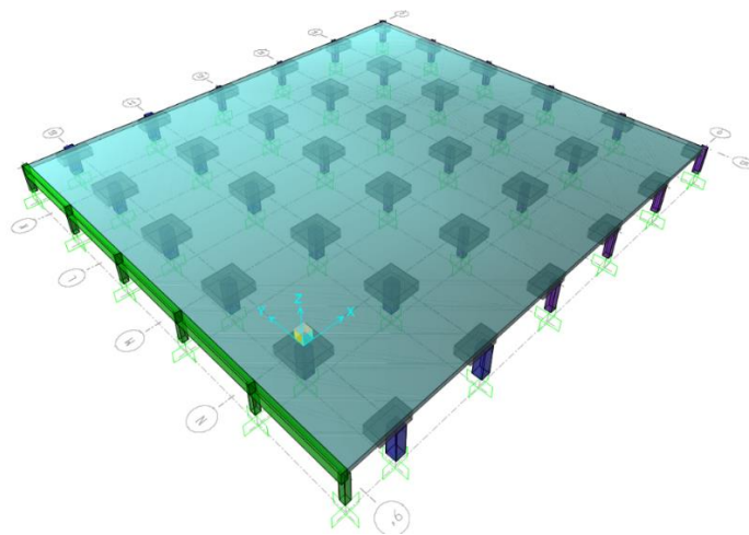
Flat slab with drop panel
