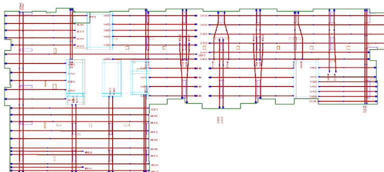
Post tension slab of building 44 story
