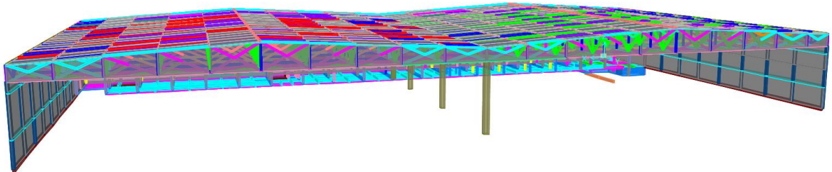
Façade Structure
