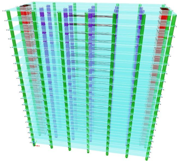
Building 20 story (Wind ឧបស.1311-50 , Earthquake ឧបស.1301/1302-61 RSA)
