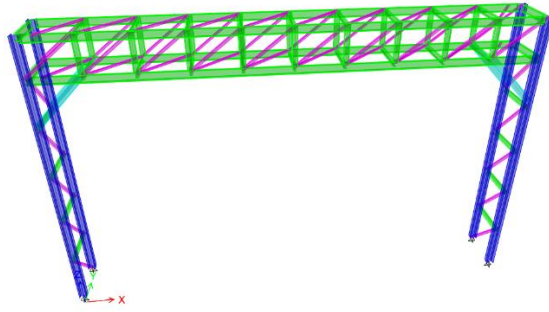
Pipe Bridge
