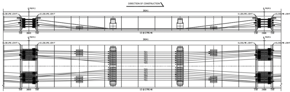
Longitudinal tendon for viaduct segment
