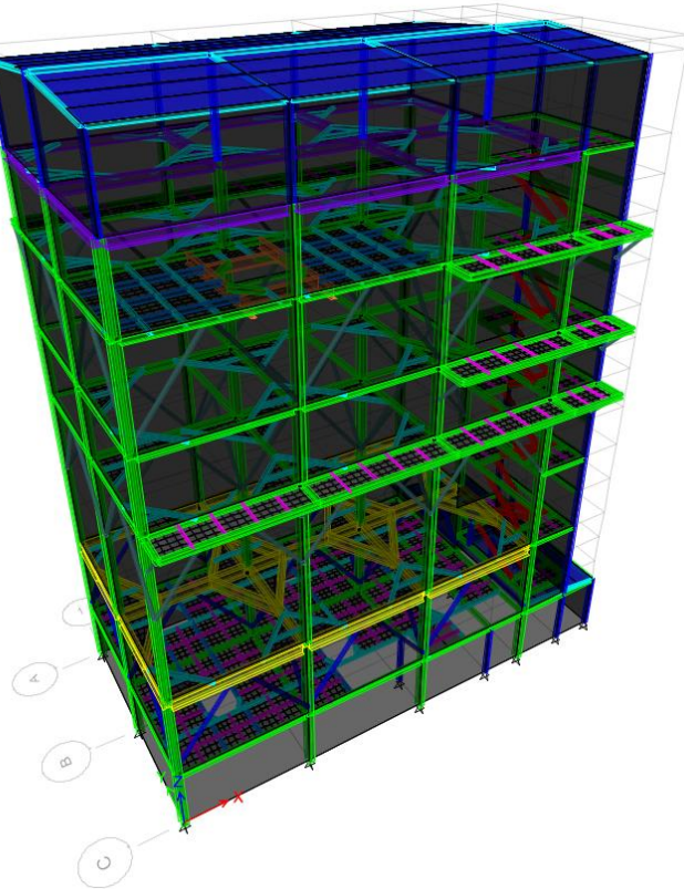
Silo Building
