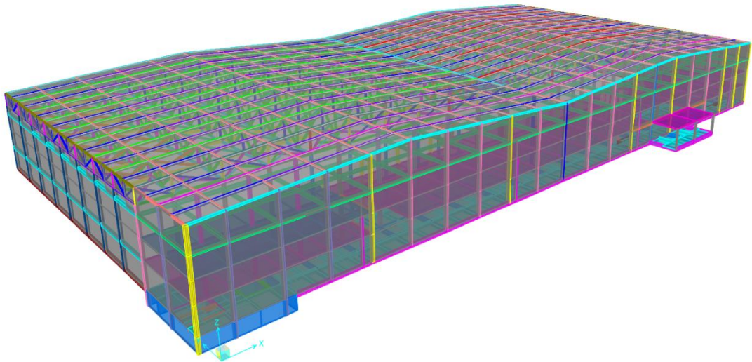
Aircraft Building
