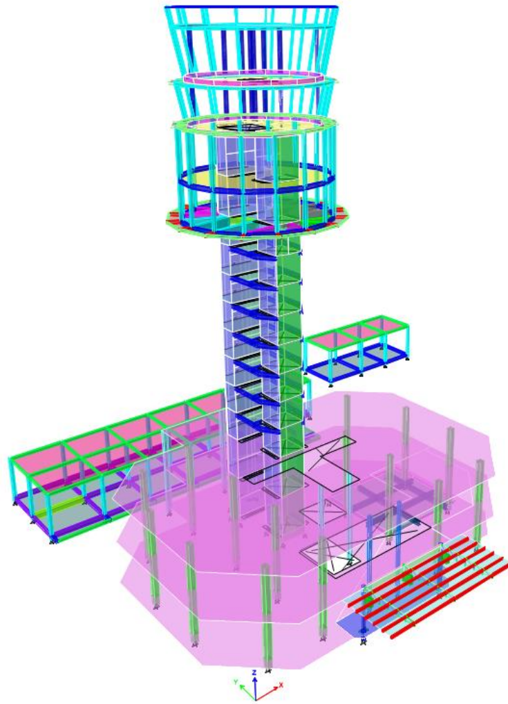
Flight control tower
