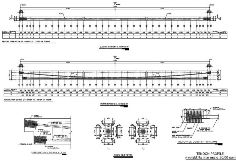
Longitudinal tendon for I Girder
