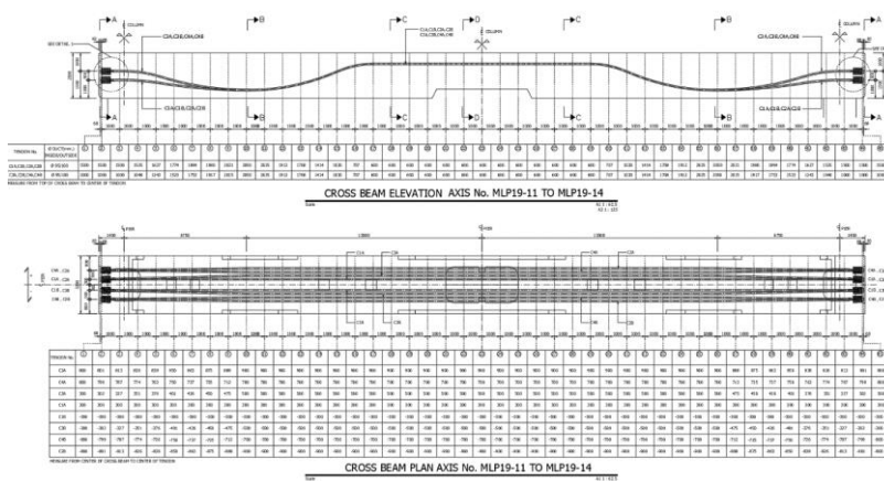
Cross Beam
