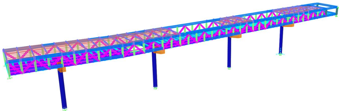
Linkage Bridge
