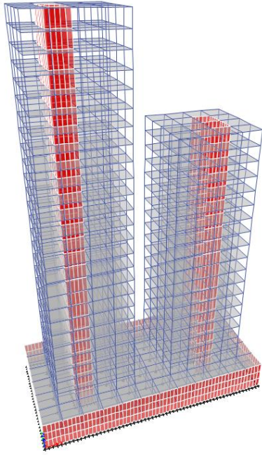
Multi Tower
