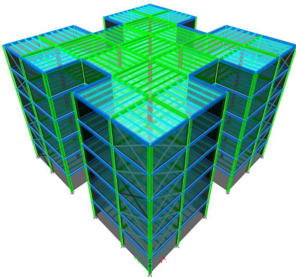
Steel Building with Composite Beam
