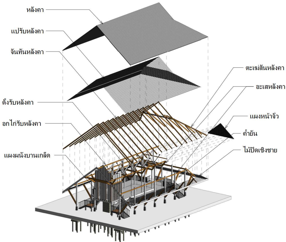
1 3D ELEMENT PRESENTATION
