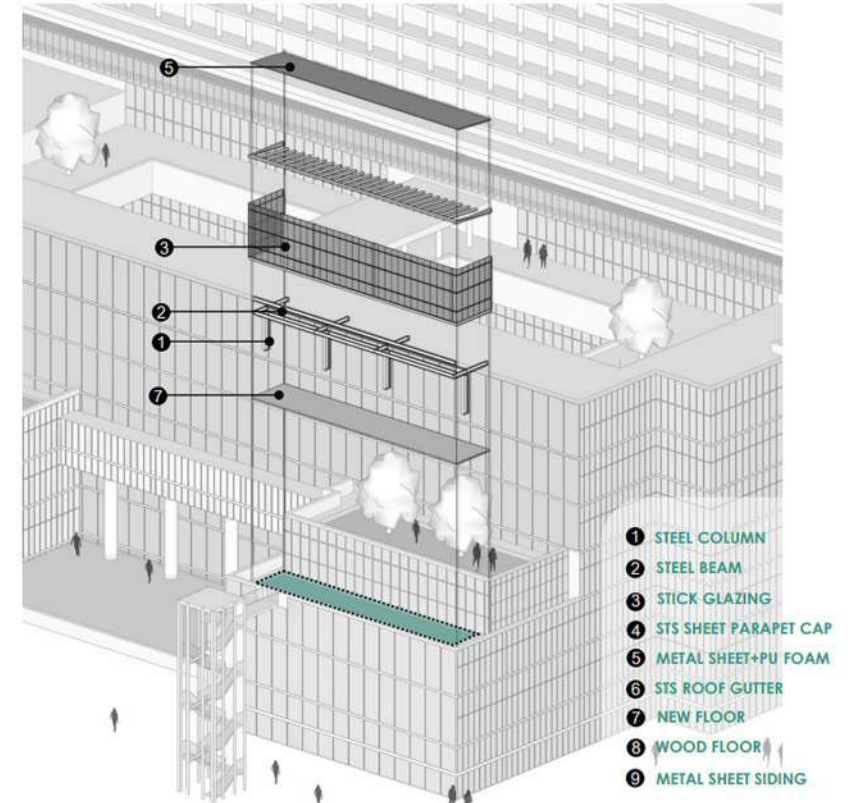
STRUCTURAL AXONOMETRIC
