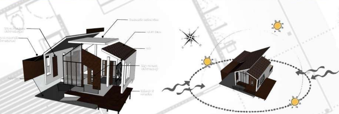
Assembly Perspective
