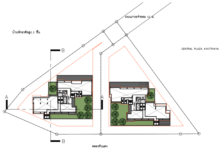
6th FLOOR PLAN SCALE A3-1 : 500
