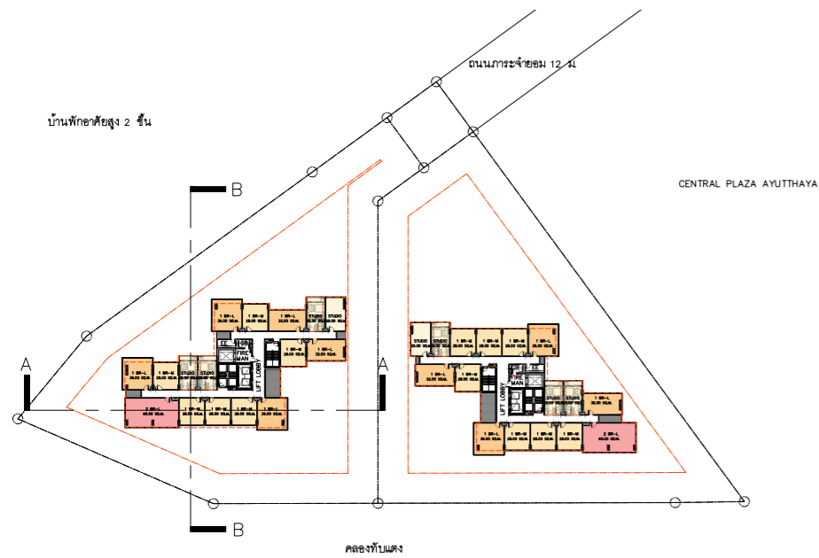
10th-19th FL PLAN SCALE A3-1 : 500
