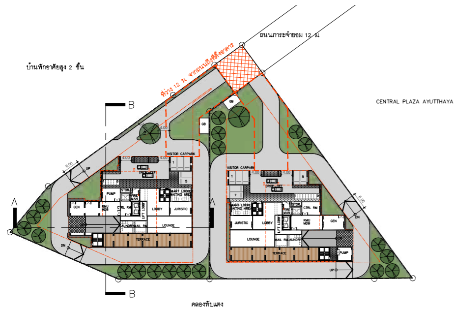
GROUND FLOOR PLAN SCALE A3-1 : 500
