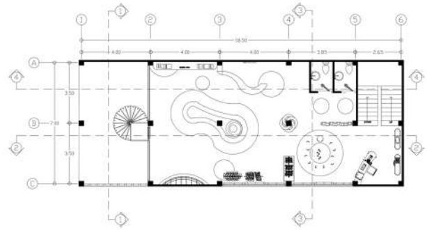
PLAN 2 FLOOR
