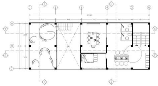
PLAN 4 FLOOR
