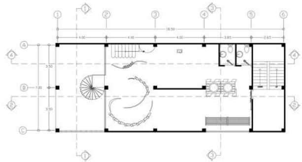
PLAN 3 FLOOR
