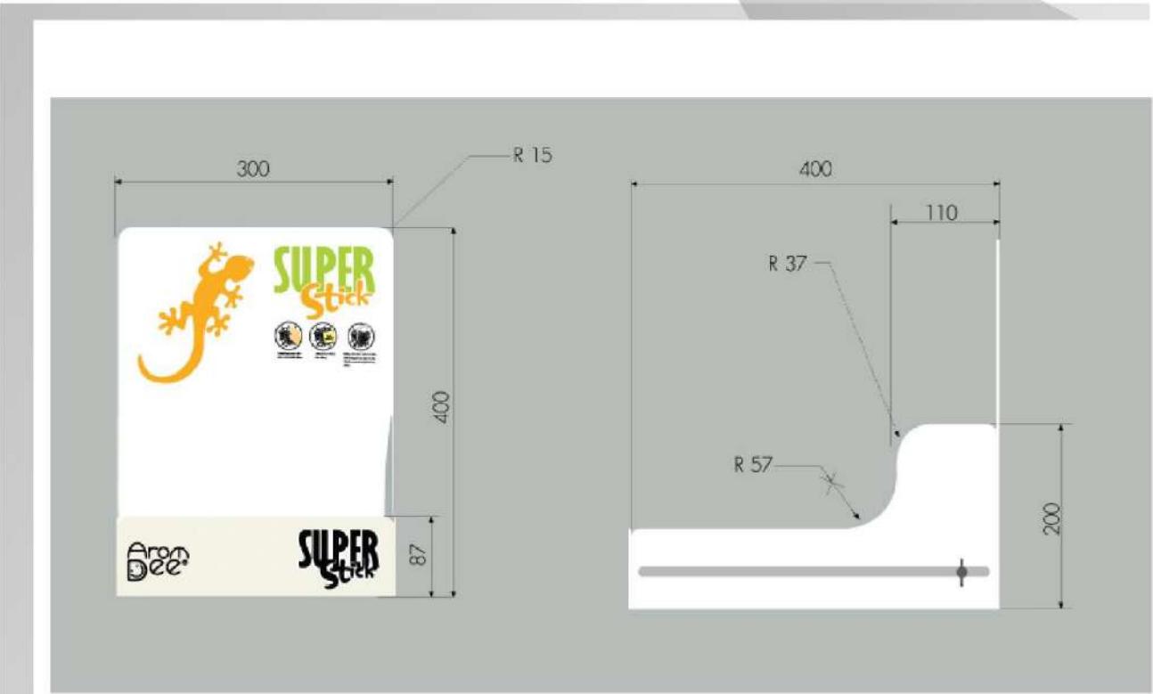
AromDee Shelf design 2
